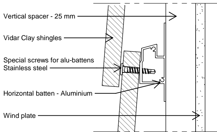
Vertical view 1 : 2
