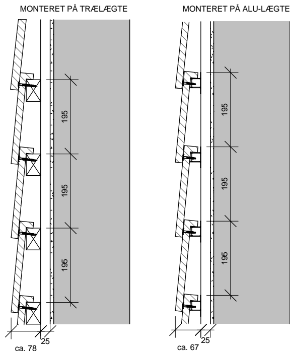
Snit 1:10
